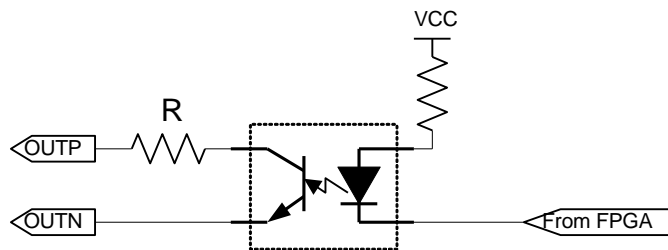
<Photo coupler output>
